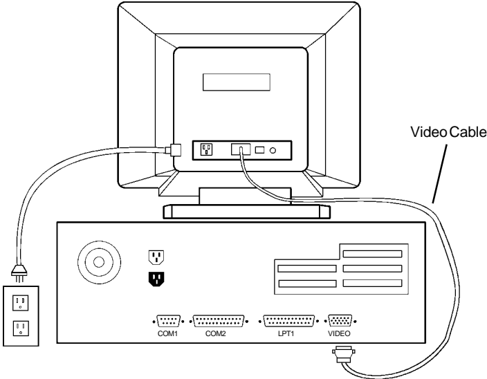
Figure 2-2 Monitor Connections
